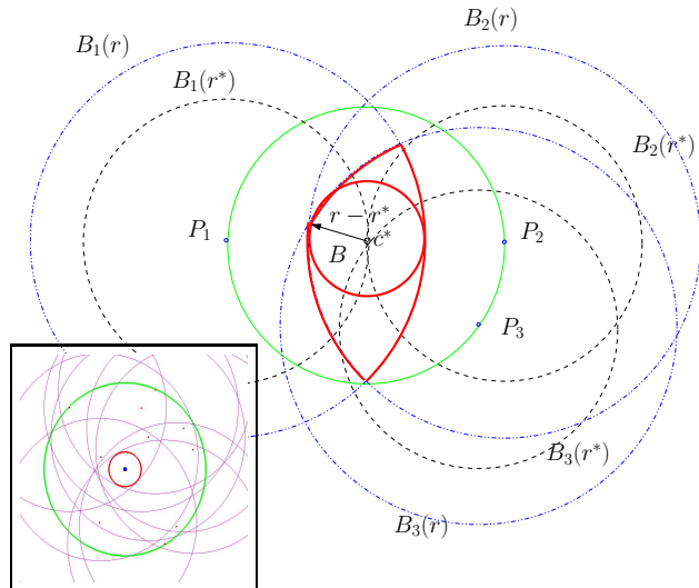
Figure 1: Covering/piercing duality for a point set. Points P_1, P_2, P_3 are associated to corresponding disks B_1(r), B_2(r), B_3(r) such that C(B_i(r)) = P_i and r(B_i(r)) = r for i \in \{1, 2, 3\} . We have B_1(r^*) \cap B_2(r^*) \cap B_3(r^*) = \{C^*\} . For r \geq r^* , there exists a disk of radius r - r^* fully contained in B_1(r) \cap B_2(r) \cap B_3(r) . Inset: SEB of 10 points (green), DP(1.2r^*) (purple) and enclosed ball (red) of radius 0.2r^* .
