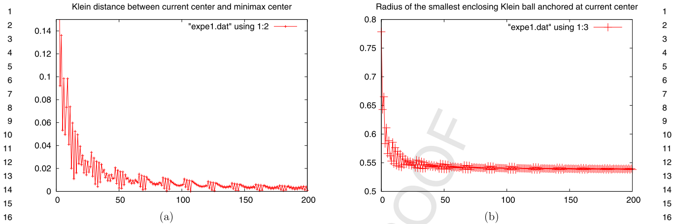
Fig. 2. Convergence rate of the GEO-ALG algorithm for the hyperbolic disk for the first 200 iterations. The horizontal axis denotes the number of iterations and the vertical axis (a) the relative Klein distance between the current center and the optimal 1-center (approximated for a large number of iterations), (b) the radius of the smallest enclosing ball anchored at the current center.
