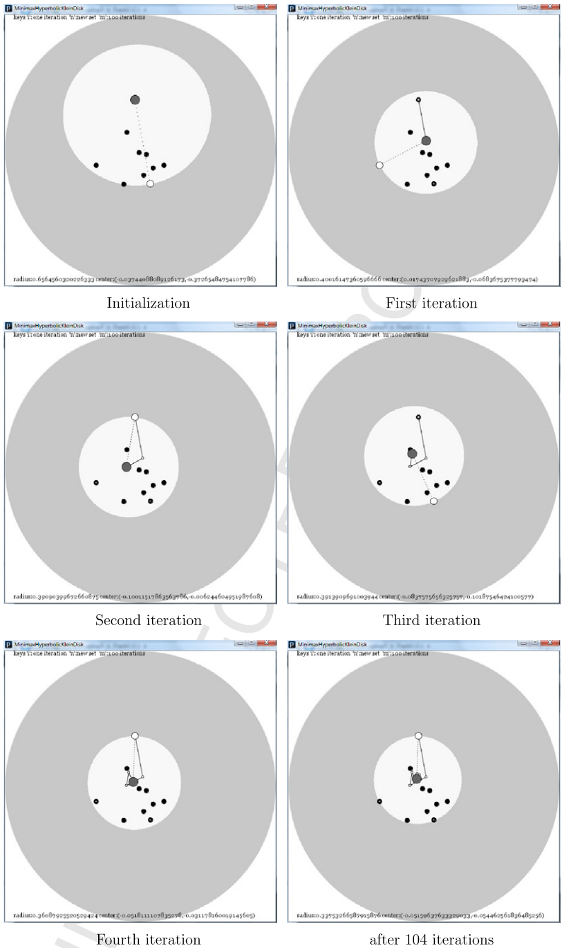
Fig. 1. Snapshots of the GEO-ALG algorithm implemented for the hyperbolic Klein disk: The large black disk and the white disk denote the current center and farthest point, respectively. The linked path shows the trajectory of the centers as the number of iterations increase. On-line demo available at http://www.informationgeometry.org/RiemannMinimax/ .
