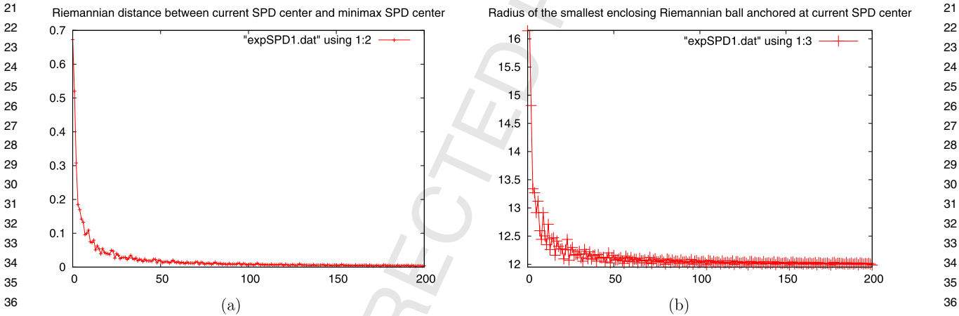
Fig. 3. Convergence rate of the GEO-ALG algorithm for the SPD Riemannian manifold (dimension 5) for the first 200 iterations. The horizontal axis denotes the number of iterations i and the vertical axis (a) the relative Riemannian distance between the current center c_i and the optimal 1-center c^* ( \frac{\rho(c_i, c^*)}{r^*} , where \rho^* and r^* are approximated for a large number of iterations), (b) the radius r_i of the smallest enclosing SPD ball anchored at the current center.
